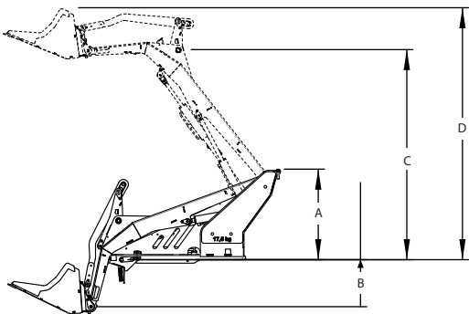
ATTACCO RAPIDO ACCESSORI quick attach attachments
